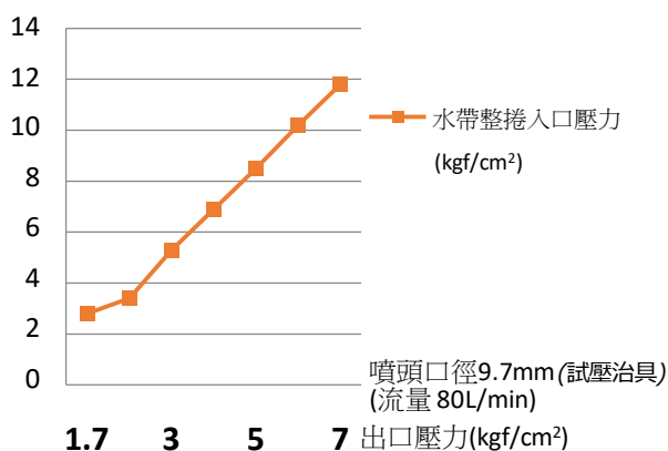
1"x30m保形水帶壓力損失
